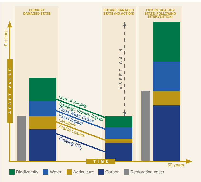
Figure 4: Comparing gains and costs in the transition between peatlands in different conditions
