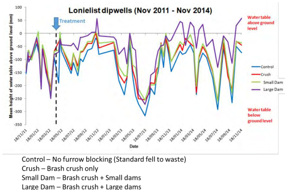
Figure G2: Monthly averaged dipwell data for brash crushing and furrow blocking monitoring experiment.
