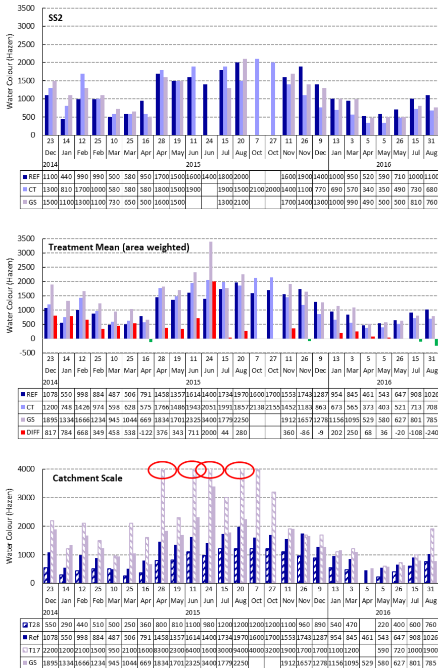
Figure F4b (i – v): The level of colour (hazen) present in water being discharged from furrows in sub-blocks (Ref, CT and GS) during regular visits to the Black Law trial site over the period December 2014 – August 2016: Climpy (graph i), SS1 (graph ii), SS2 (graph iii), all blocks combined (graph iv) and concentrations at catchment scale (graph v). See Figure legend 18a for further details.
