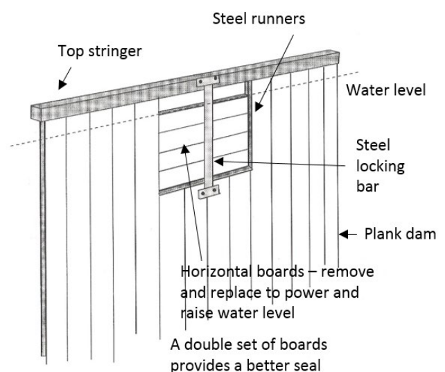
Figure 107 Plank dams can be modified to incorporate an adjustable sluice at the spillway to give a greater degree of water level control.
