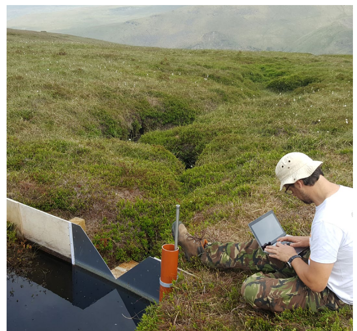
Figure 81 A plywood dam is prone to rotting at the air/water/peat interface. If the water level can be maintained at the bog surface and Sphagnum quickly recolonised, rotting is reduced © Emma Shuttleworth
