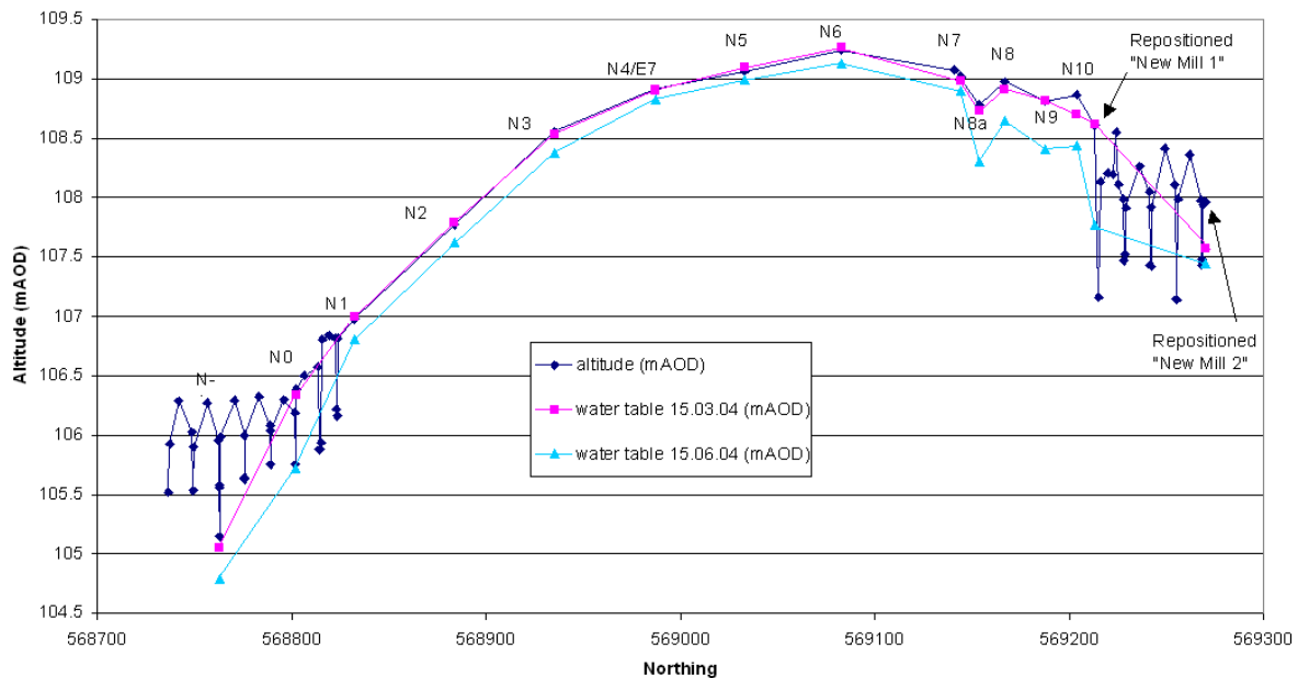
Figure 15 Impact of drainage ditches on water tables on a cut-over raised bog
